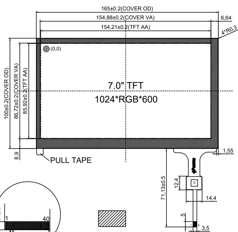
BLACK:RAL9005 Front view
