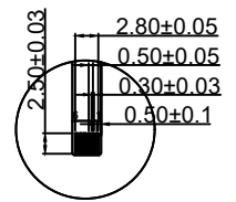
DETAIL "B" 2:1
